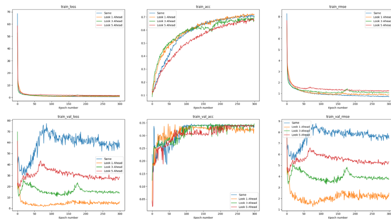
Figure 3. MSE loss, Accuracy and RMSE for the dense networks on both the train and test datasets.
