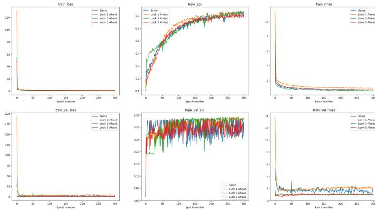
Figure 2. MSE loss, Accuracy and RMSE for the LSTM networks on both the train and test datasets.
