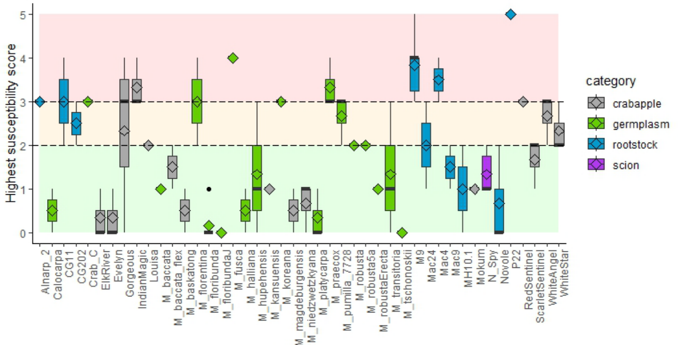
Figure 4- Boxplot of highest recorded susceptibility score across all scoring events pre- and post inoculation(s). The mean highest score is indicated by diamonds. Arbitrary category of susceptibility is indicated by red, orange, and green areas, representing susceptible, intermediate, and resistant categorisation, respectively.
