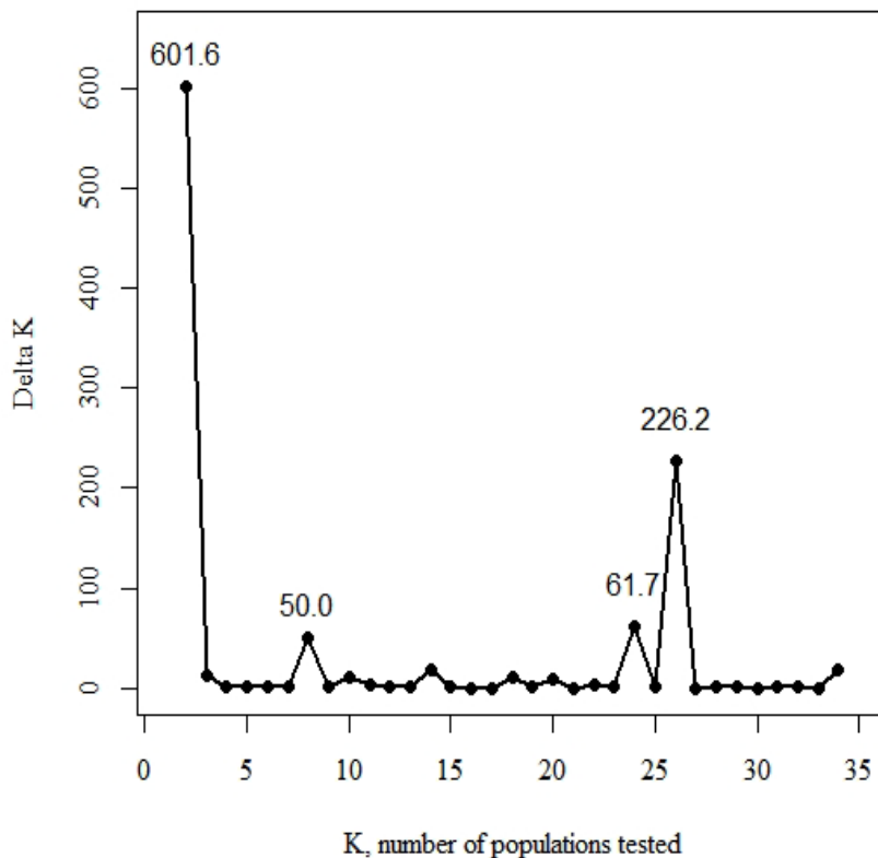
Figure 5- Likelihood (delta K), of the number of genetic populations (K) being present within the woolly apple aphid samples analysed with SSR markers.
