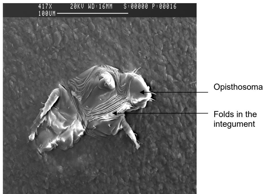
Figure 1.3a.: Dorsal view of an adult female, showing patterning in the integument similar to the folds seen in smaller larvae and a much reduced opisthosoma (the hind part of the body behind the legs)
