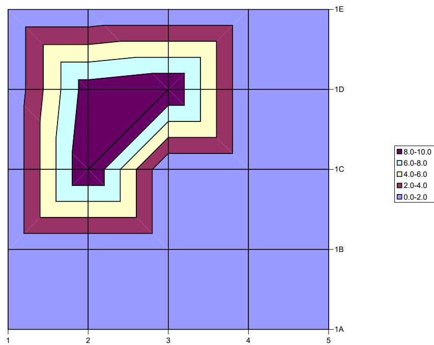
Figure 2.6: Two examples of the distribution of feeding marks (as the percentage of damaged bulbs in 5 x 5 grids) from samples taken in 2008.
